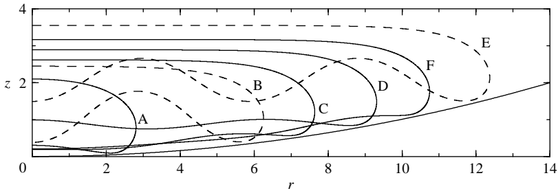
FIGURE 3. Shapes corresponding to the labelled points on figure 2. Shapes B and E (dashed) have large oscillations on the lower surface and appear unlikely to be stable.
