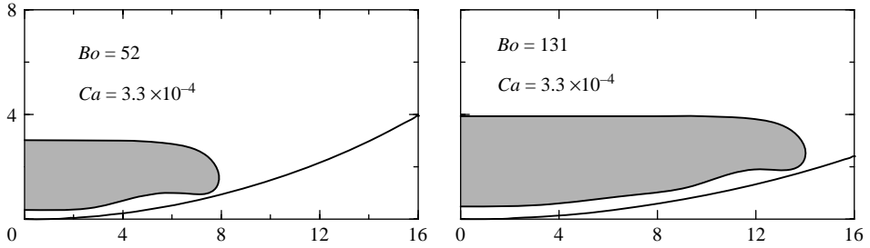
FIGURE 5. Typical comparison between stable Navier–Stokes POLYFLOW simulations (grey shapes) and our lubrication results (solid lines) for two values of Bo = \rho g V^{2/3}/\sigma .
