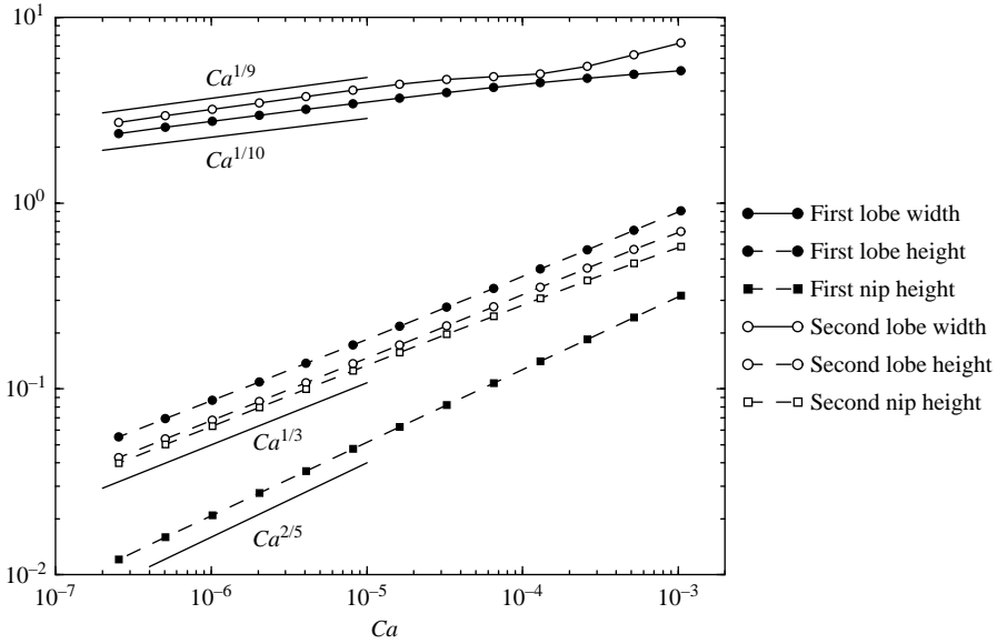
FIGURE 8. The dimensions of the first two nips and lobes from the numerical solution of (2.8), for R_p = 13.73 and Bo \approx 130 . The heights of the nips and lobes are the minima and maxima of h(r) respectively; the widths of the lobes are defined by the horizontal distance between two successive nips. The height of the first nip scales like Ca^{2/5} , as predicted; the scalings of subsequent lobes and nips are indistinguishable from the asymptotic predictions of Ca^{1/3} and Ca^{1/10} .
