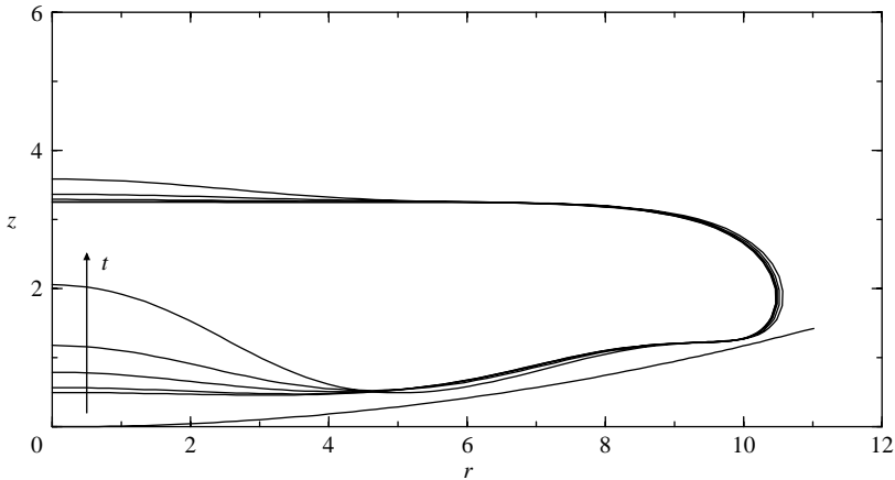
FIGURE 6. Time-dependent simulation with POLYFLOW. An unstable case, with Ca = 6.7 \times 10^{-5} and Bo = 82 .
