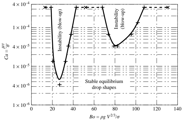
FIGURE 7. Stability diagram obtained from the POLYFLOW simulations (Lange 2002). The symbols + and \times mark stable simulations; instability is manifested by growth of a central air bubble (figure 6).
