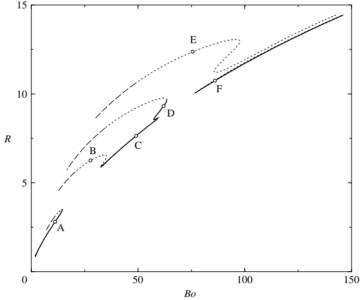
FIGURE 2. Radius of the drop R as a function of the Bond number for Ca = 3.59 \times 10^{-5} in a spherical mould of radius a_M = 50 . The shapes corresponding to the labelled points are shown in figure 3. The dashed parts of the curves correspond to unphysical shapes that self-intersect. The dotted parts correspond to shapes with large-amplitude waves on the lower surface, which are unlikely to be stable. The solid parts correspond to the smallest vertical offset h_p for a given value of Bo , give reasonable shapes and are most likely to be observed.
