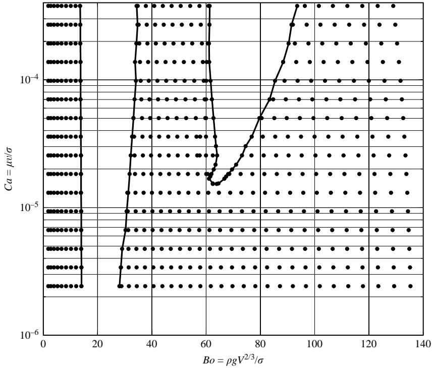
FIGURE 4. Regime diagram obtained from the lubrication solutions. The solid circles correspond to solution branches A, C, D and F (figure 2).
