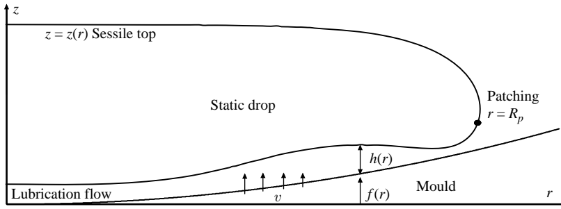
FIGURE 1. Sketch of the problem. Air is injected through the mould with Darcy velocity v . Solutions for the sessile top surface and the lubrication layer beneath are patched at r = R_p , and the maximum radius is r = R . We non-dimensionalize lengths with the capillary length l_c = (\sigma/\rho g)^{1/2} , so that the dimensionless top surface is given by \kappa(r) - z(r) = \kappa(0) .
